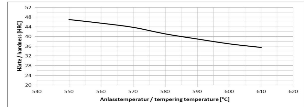
Tempering diagram: Average values on samples dia 25 mm x length 50 mm
